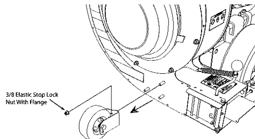
Figure 1. Removing Original Wheel
