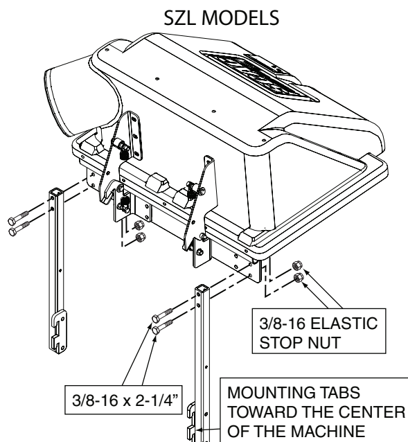
Figure 2-15. Up Tube Installation
