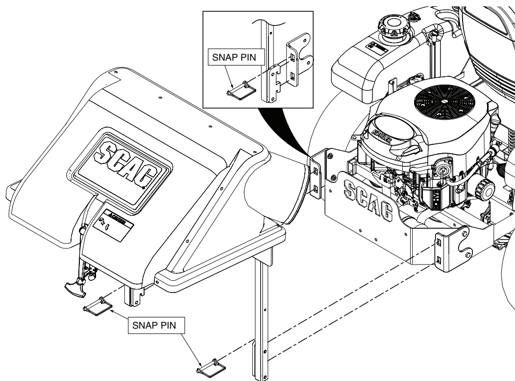
Figure 2-18. SZL Hopper Mounting Holes
