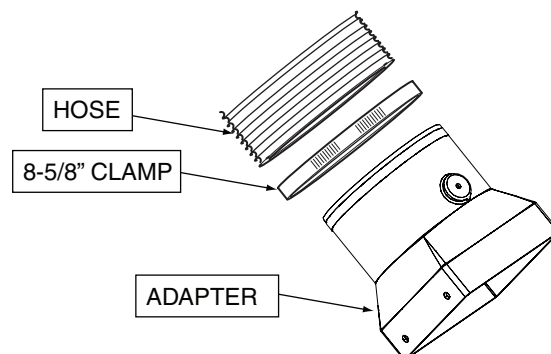
Figure 2-16. Hose to Adapter Installation
