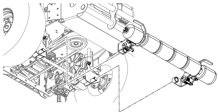
Figure 2-8. Install Roller Assembly
