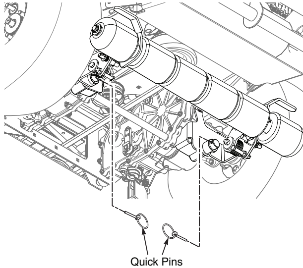
Figure 2-9. Install Quick Pins
