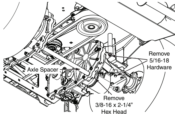
Figure 2-1. Remove Hardware
