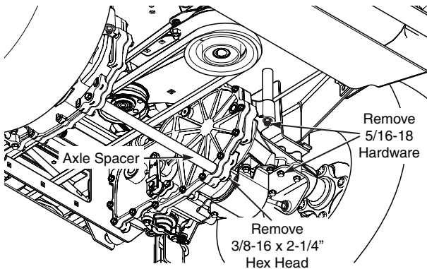
Figure 2-6. Remove Hardware
