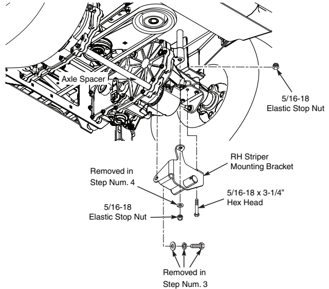
Figure 2-7. Install RH Striper Mounting Bracket
