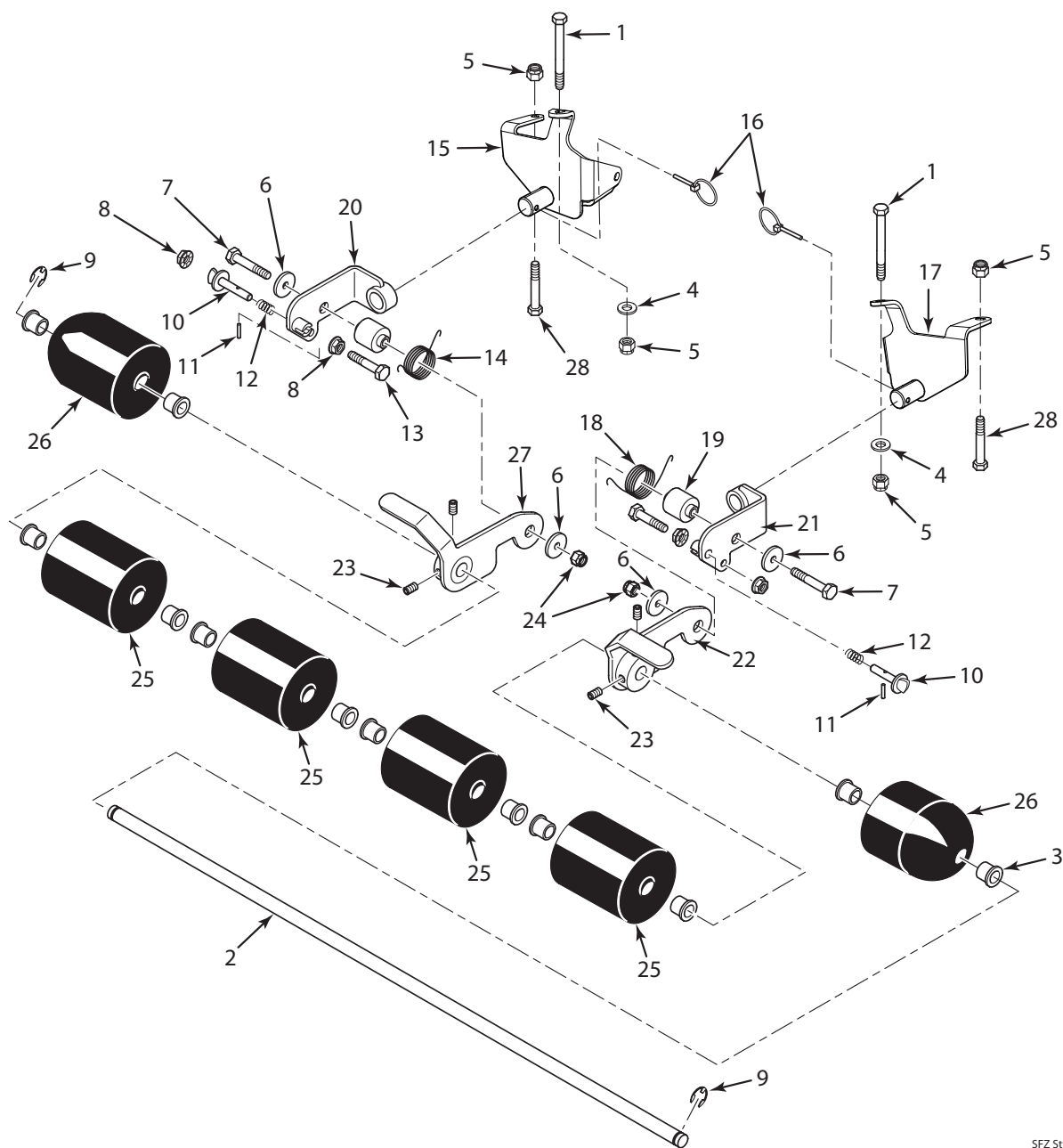
SFZ Striper Exploded View
