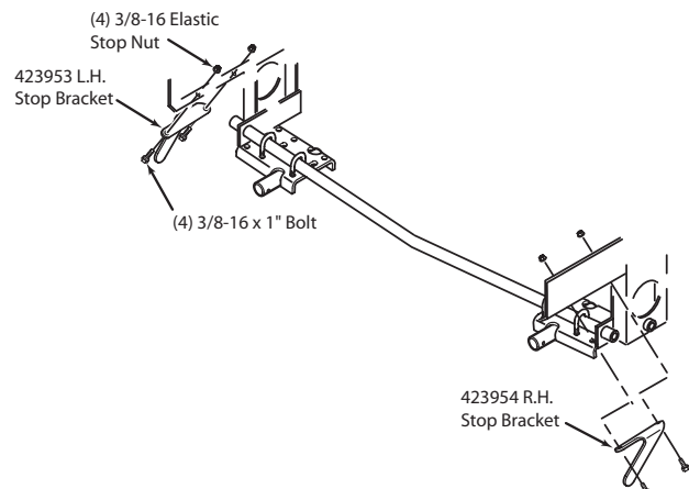
Figure 2-14. Install Striper Stop Brackets
