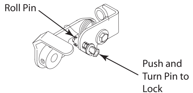
Figure 3-5. Locking Roller in Transport Position
