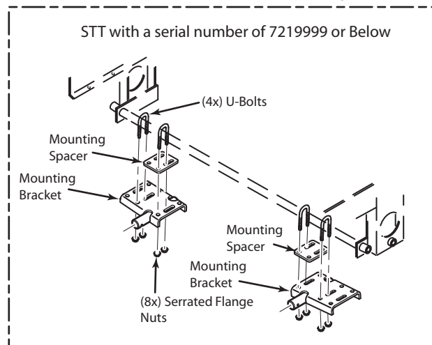
Figure 2-13. Mounting Bracket Install
