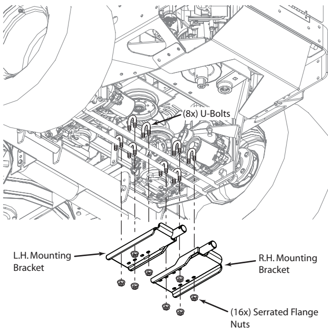
Figure 2-10. Mounting Bracket Install
