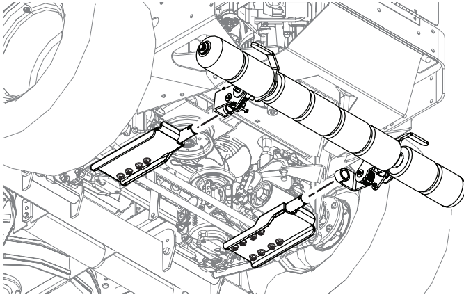
Figure 2-12. Install Roller Assembly
